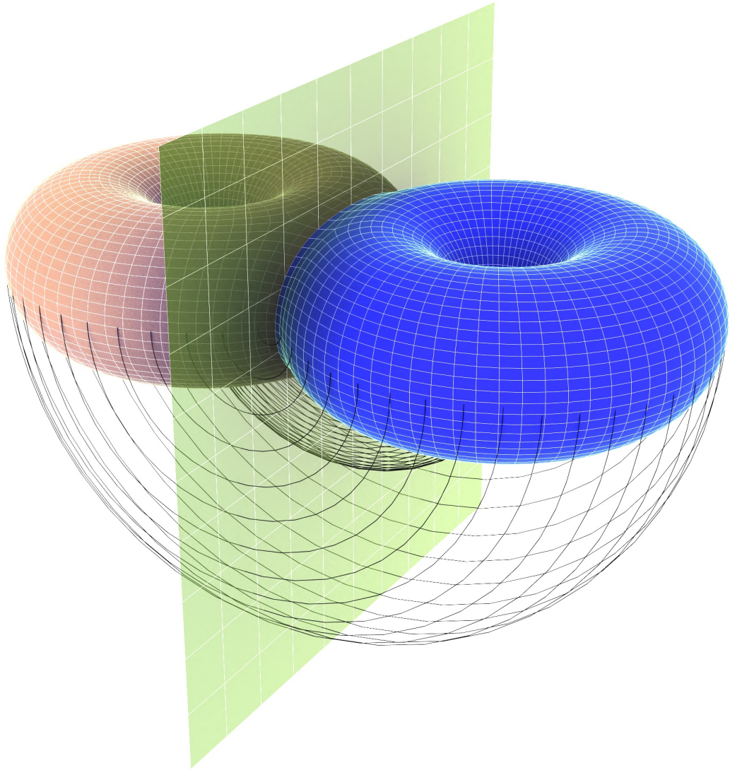
Figure 0.1: The double of the blue manifold with boundary is nullbordant. This can be seen by following the movement of a rotation by 180^\circ to its reflection along the hyperplane as pictured. This traces out a manifold one dimension higher bounding the blue and pink manifold glued together.
