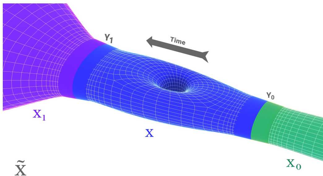
Figure 5.2: A picture of a bordism \tilde{X} in a definition that is more suitable for generalizations to non-topological functorial quantum field theories, following Stolz-Teichner [72, 73]. The middle blue region X is called the core and should be thought of as the ‘actual bordism’. The incoming green region X_0 and outgoing purple region X_1 stretch out to infinity and should be thought of as ‘redundant data’. The bordism goes from the object Y_0 , which comes equipped with little collar Y_0 \times (-\epsilon_0, \epsilon_0) , to the collar Y_1 \times (-\epsilon_1, \epsilon_1) . These collars lie partially inside the core and partially outside as pictured.
