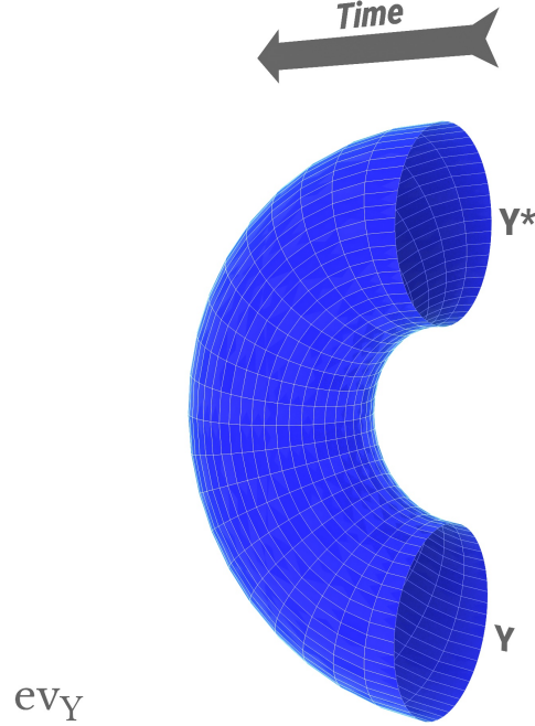
Figure 1.1: The macaroni bordism from the disjoint union of the space Y and its dual Y^* . It is the evaluation map \text{ev}_Y realizing Y^* as the dual of Y in the bordism category.
