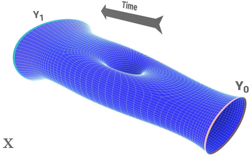
Figure 5.1: An n -dimensional bordism X from the (n - 1) -dimensional manifold Y_0 to the (n - 1) -dimensional manifold Y_1 .
